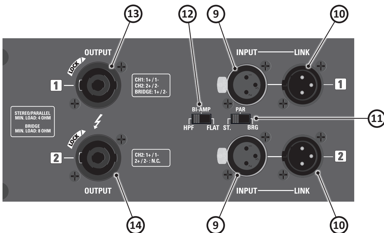
REAR PANEL (FIG.5)
